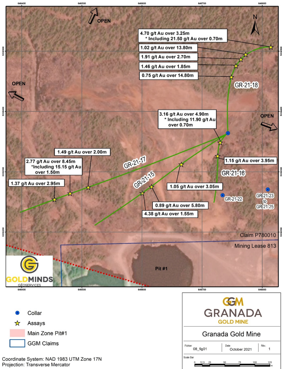
Figure 1: Plan Map Showing Drill Hole and Assay Locations immediately North of Pit #1.
