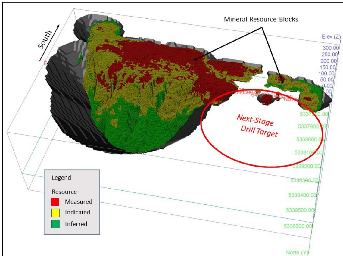
Figure 1. Perspective 3D Image of Resource Blocks of the Pit-Constrained Current Resources at the Granada Gold Project (Looking roughly South).
